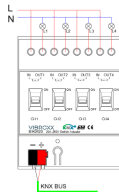
Wiring diagram
